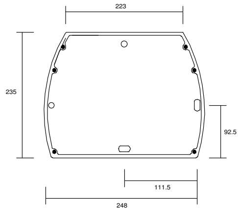
Diagram 2: Fixing details
